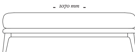
Banqueta 1070x1070x460mm
